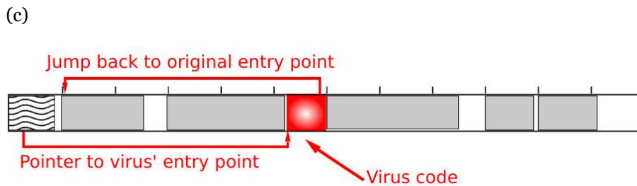
Fig. 13.4: Placement of virus code in an executable file.
