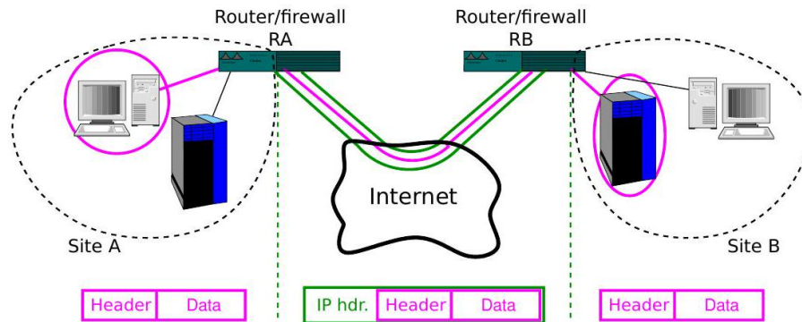
Fig. 11.8: Site-to-site tunneling
